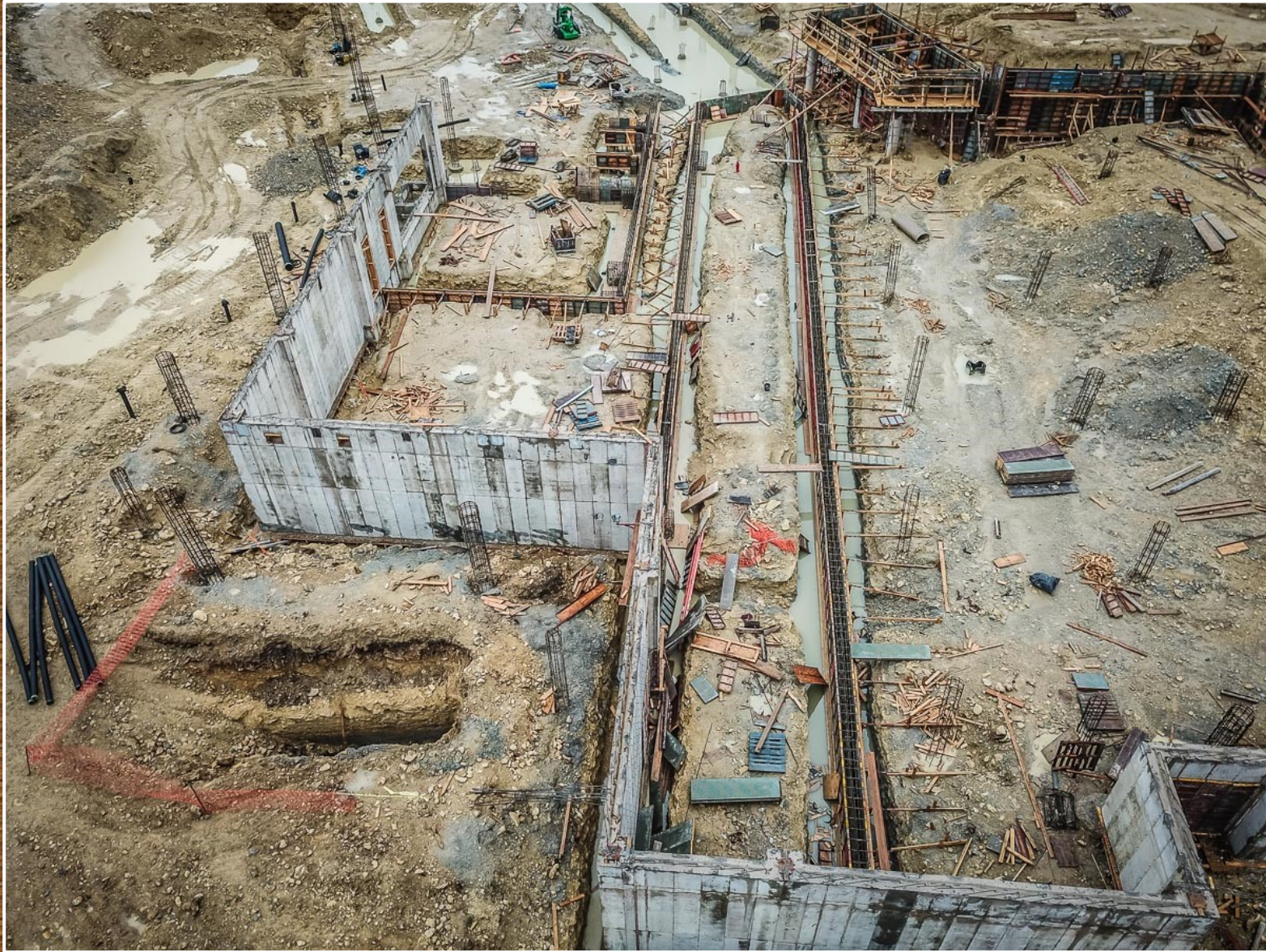
Eastern walls in the business area are being formed up for future concrete pour.
